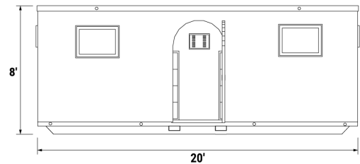
COLLAPSIBLE MODULAR UNIT FRONT VIEW
