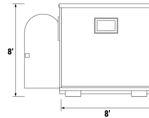
COLLAPSIBLE MODULAR UNIT RIGHT SIDE VIEW
