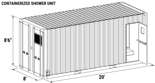
CONTAINERIZED SHOWER UNIT
