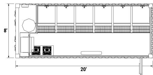
CONTAINERIZED SHOWER UNIT TOP VIEW
