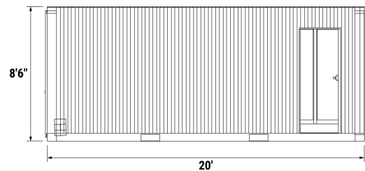
CONTAINERIZED SHOWER UNIT FRONT VIEW
