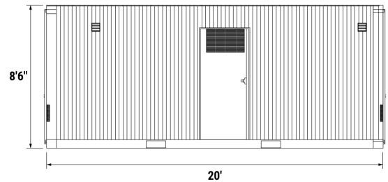
CONTAINERIZED LAUNDRY UNIT FRONT VIEW
