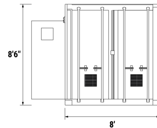
CONTAINERIZED LAUNDRY UNIT RIGHT SIDE VIEW
