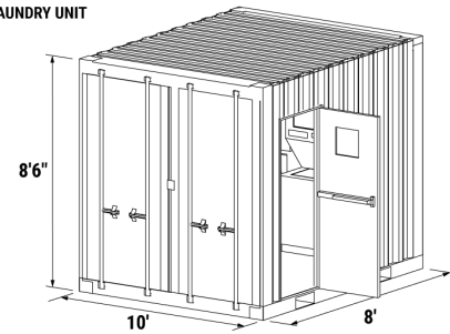
BICON LAUNDRY UNIT FRONT VIEW
