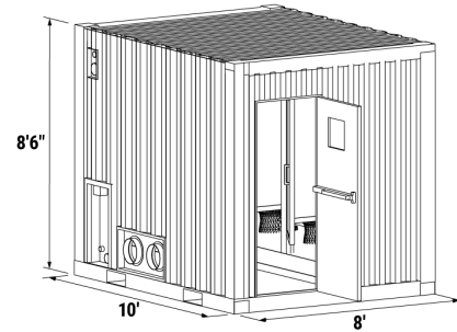
BICON TOILET UNIT FRONT VIEW
