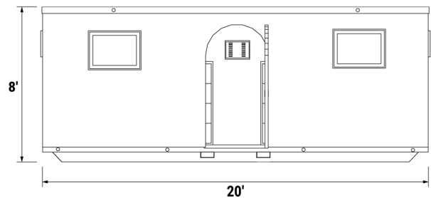
COLLAPSIBLE MODULAR OFFICE UNIT FRONT VIEW
