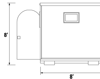
COLLAPSIBLE MODULAR OFFICE UNIT RIGHT SIDE VIEW
