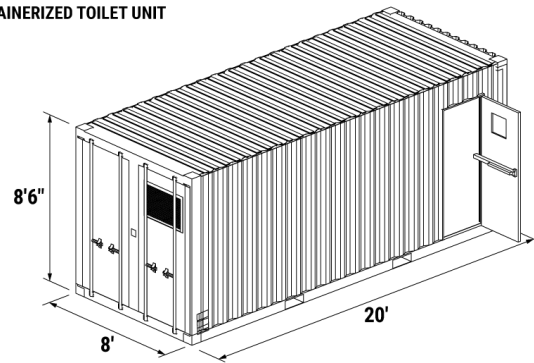
CONTAINERIZED TOILET UNIT
