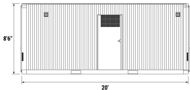
CONTAINERIZED LAUNDRY UNIT FRONT VIEW
